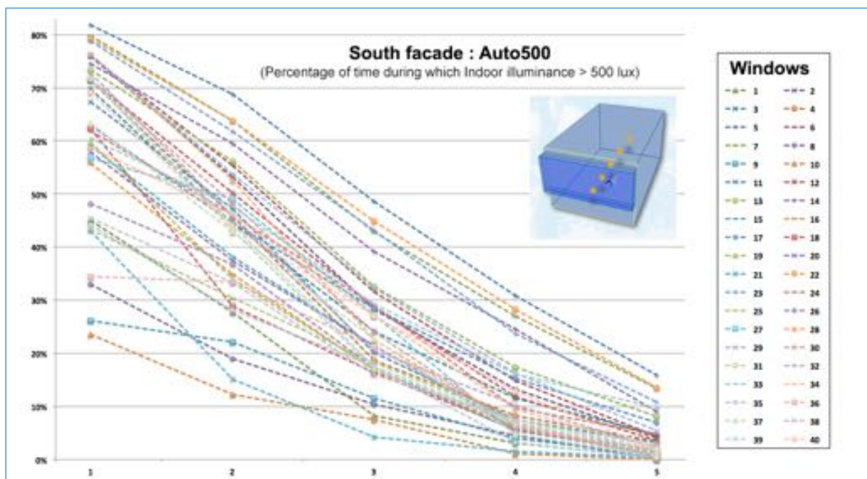
Figure 9: Percentage of the time (7 AM- 6 PM), during which daylight contribution \geq 500 lux on the five reference points, for each of the 40 south oriented rooms. Each line correspond to a room. Point 1 (left), is located close to the window and point 5 (right) is at the back of the room.
