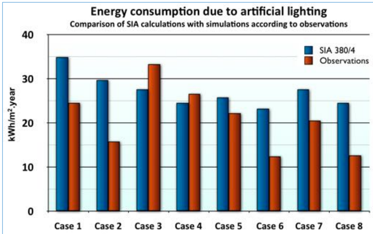
Figure 11: Energy consumption for lighting: comparison between the calculations with the Swiss Standard SIA 380/4 (blue) and the simulations based on observations (red, median values).
